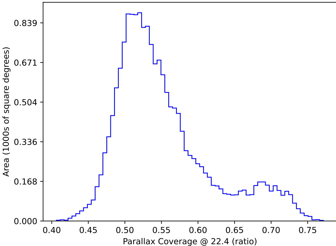
baseline_v2.0_10yrs WFD: Parallax Coverage @ 22.4
