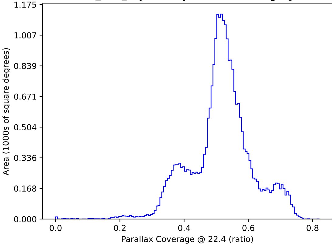
baseline_v2.0_10yrs All sky: Parallax Coverage @ 22.4
