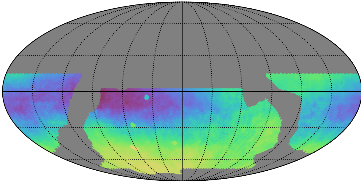
baseline_v2.0_10yrs WFD: Parallax-DCR degeneracy @ 24.0
