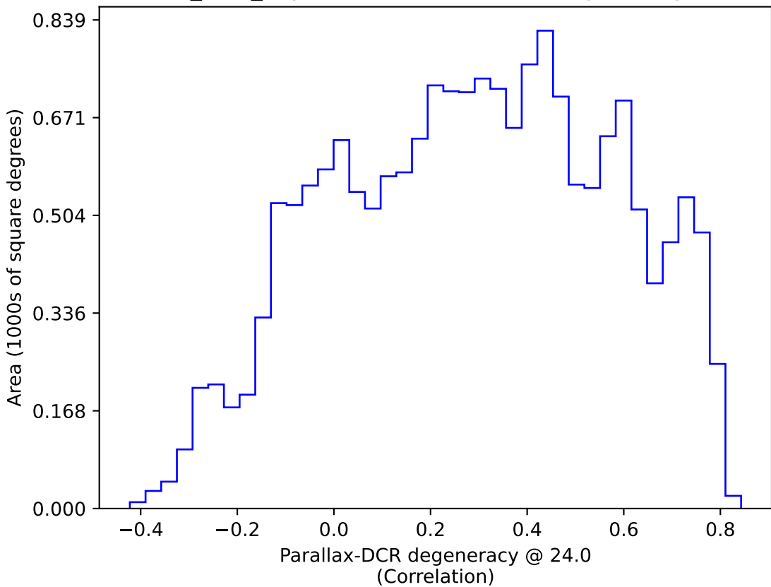
baseline_v2.0_10yrs WFD: Parallax-DCR degeneracy @ 24.0
