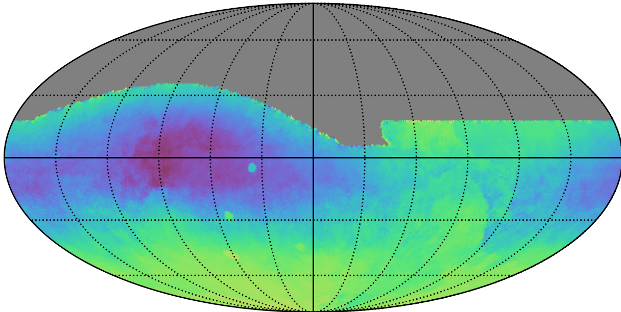
baseline_v2.0_10yrs All sky: Parallax-DCR degeneracy @ 24.0
