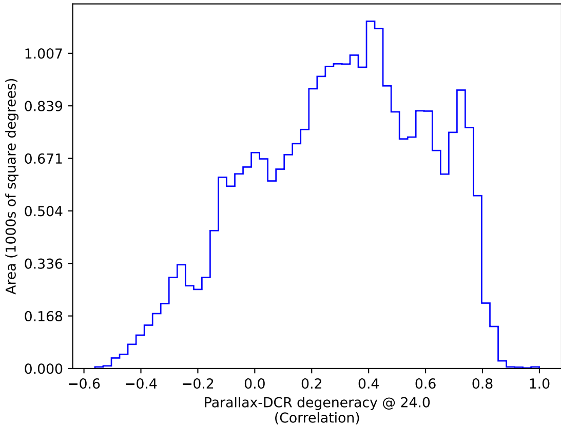
baseline_v2.0_10yrs All sky: Parallax-DCR degeneracy @ 24.0
