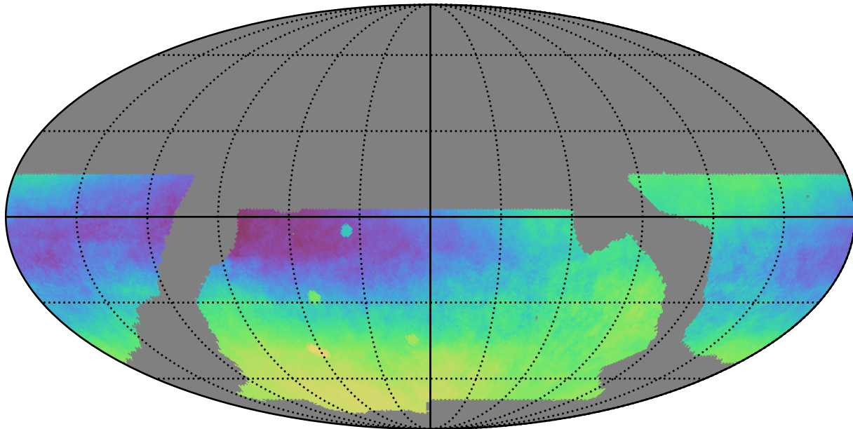
baseline_v2.0_10yrs WFD: Parallax-DCR degeneracy @ 22.4
