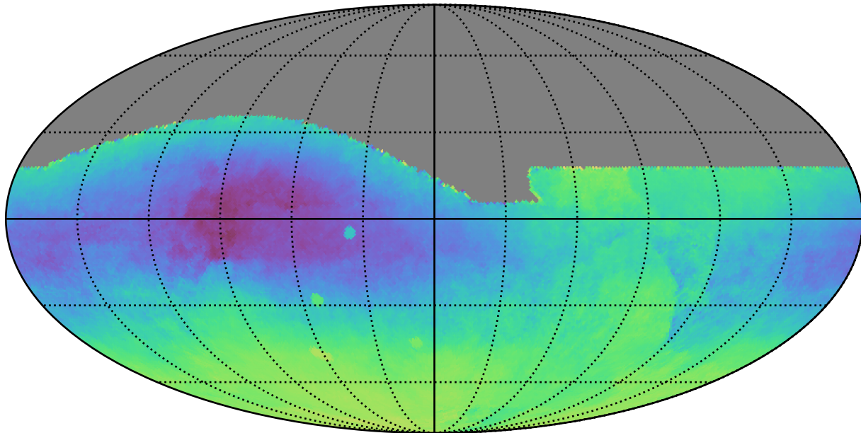
baseline_v2.0_10yrs All sky: Parallax-DCR degeneracy @ 22.4
