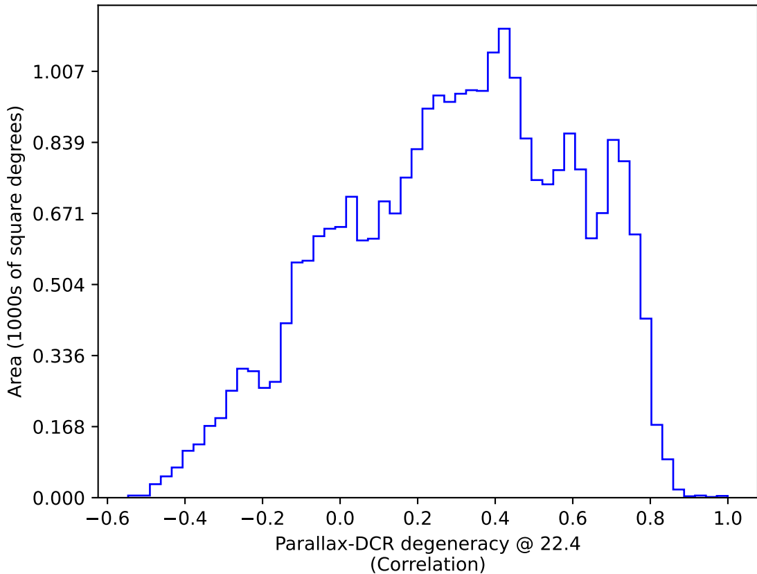
baseline_v2.0_10yrs All sky: Parallax-DCR degeneracy @ 22.4
