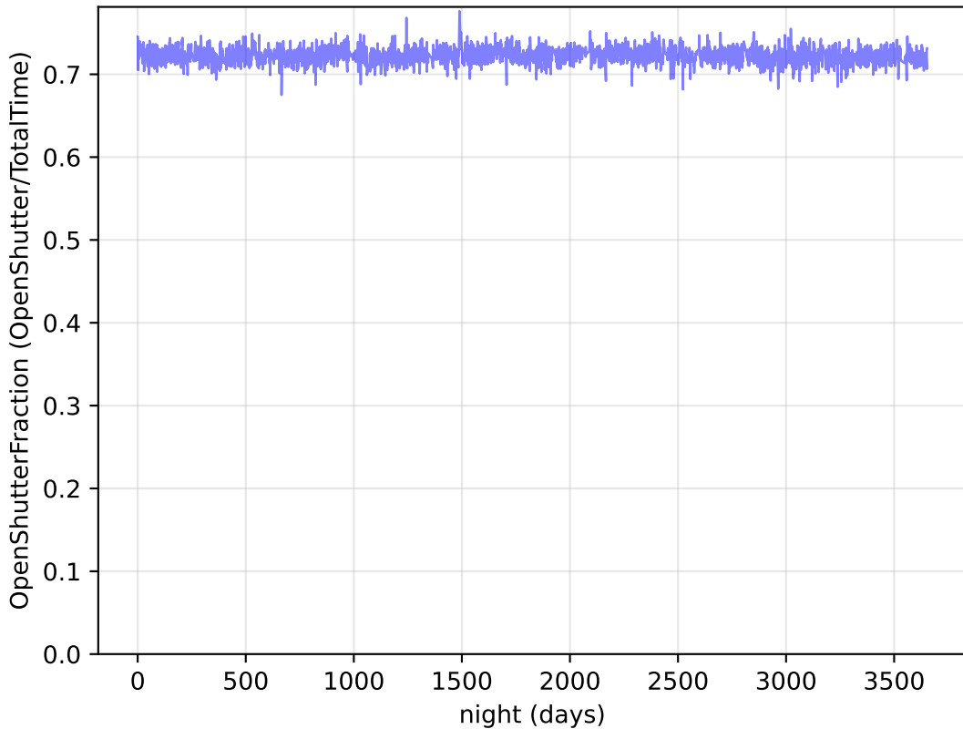
baseline_v2.0_10yrs Per night: OpenShutterFraction
