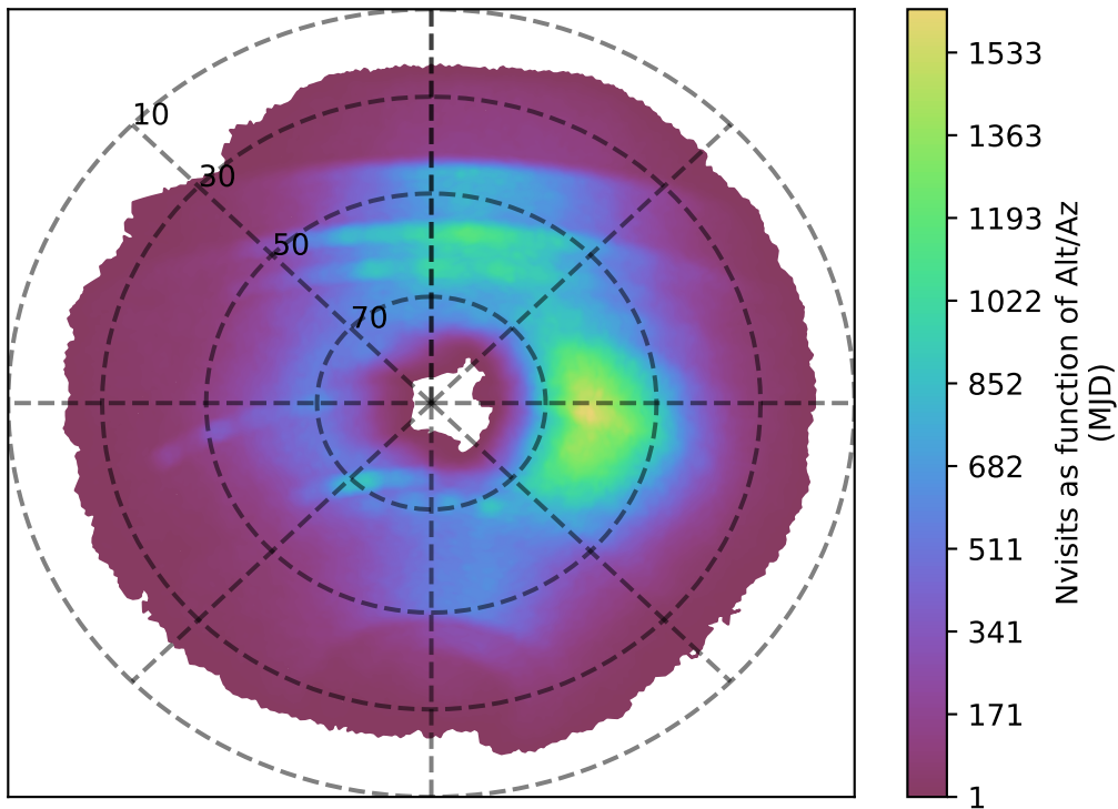
baseline_v2.0_10yrs z band: Nvisits as function of Alt/Az
