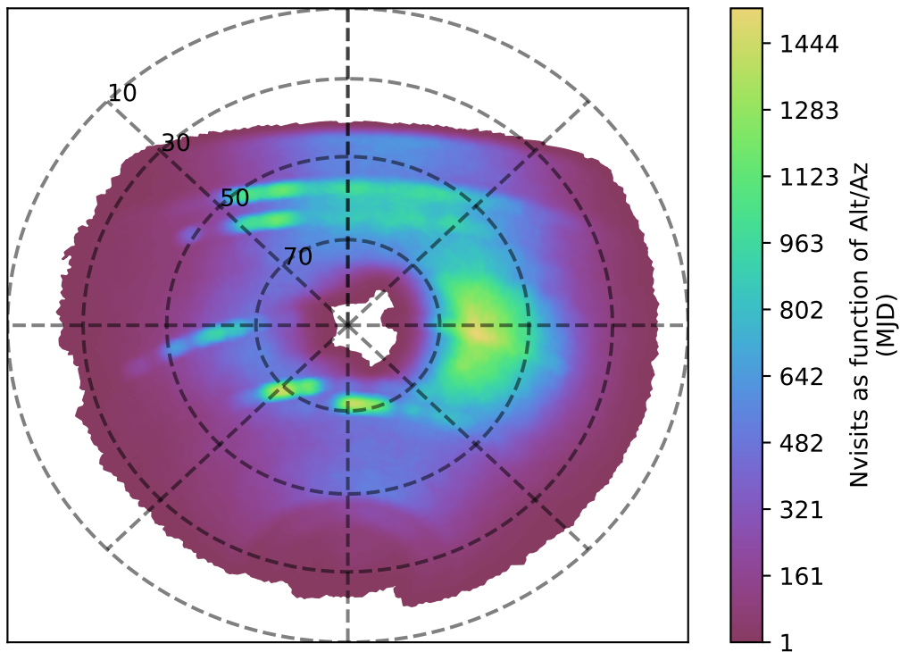
baseline_v2.0_10yrs y band: Nvisits as function of Alt/Az
