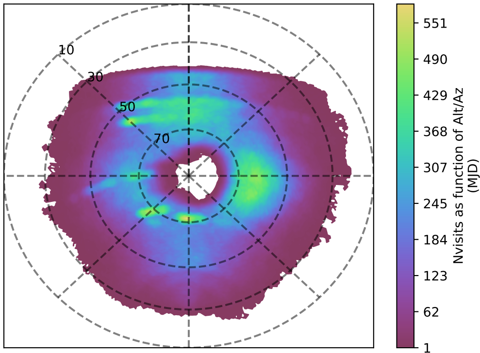
baseline_v2.0_10yrs u band: Nvisits as function of Alt/Az
