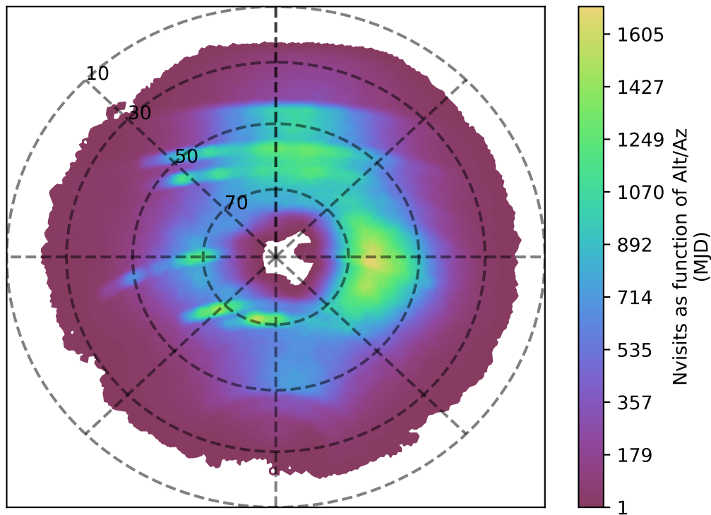
baseline_v2.0_10yrs r band: Nvisits as function of Alt/Az
