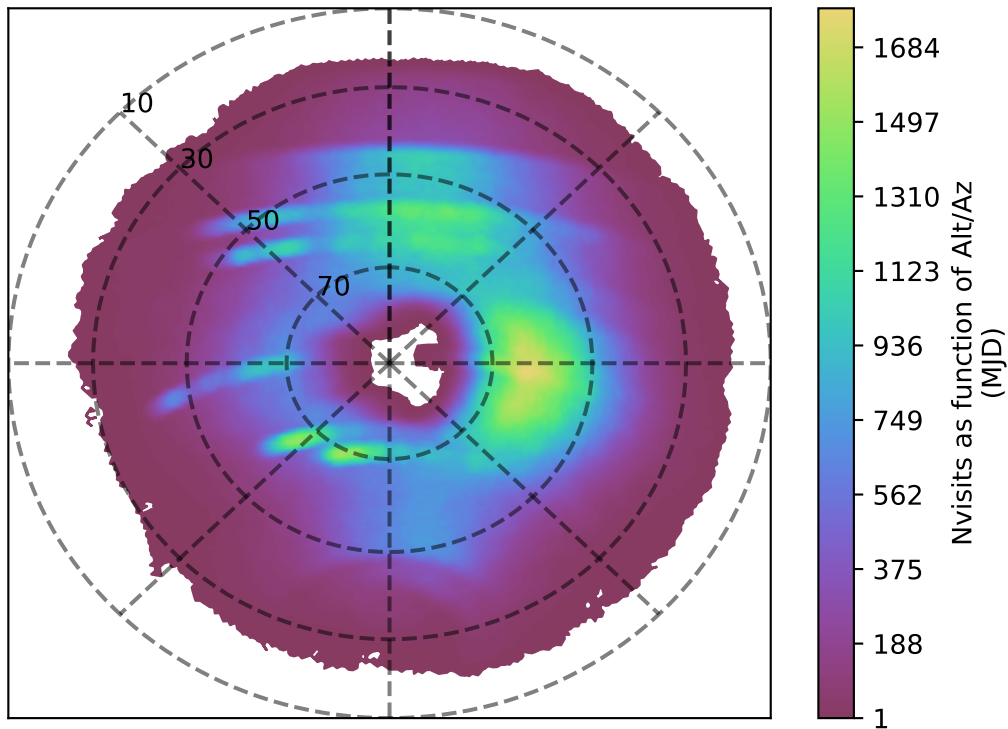
baseline_v2.0_10yrs i band: Nvisits as function of Alt/Az
