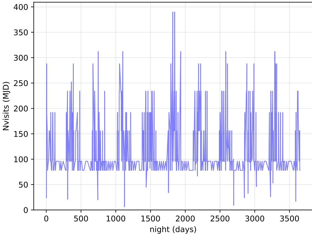
baseline_v2.0_10yrs DDF: Nvisits
