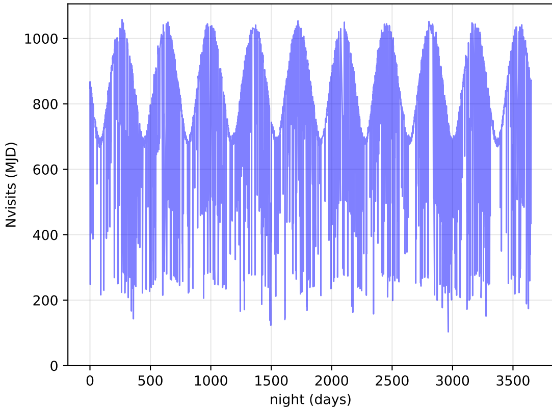
baseline_v2.0_10yrs All visits: Nvisits
