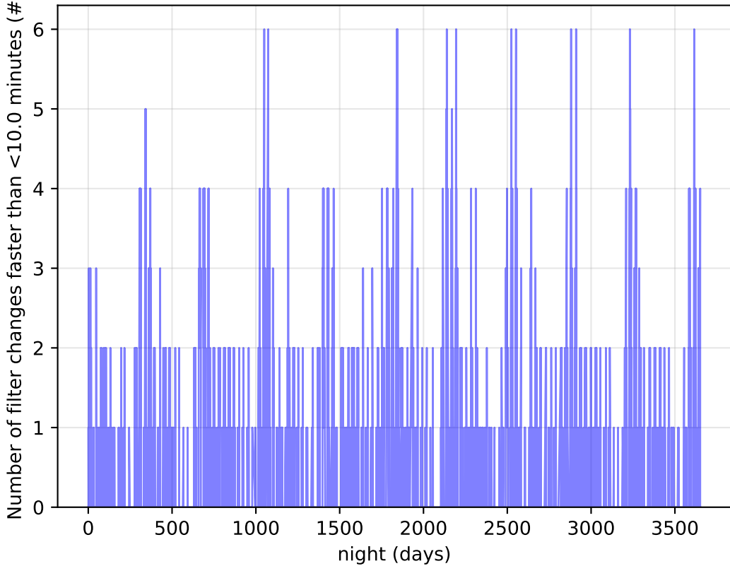
baseline_v2.0_10yrs Per Night: Number of filter changes faster than <10.0 minutes
