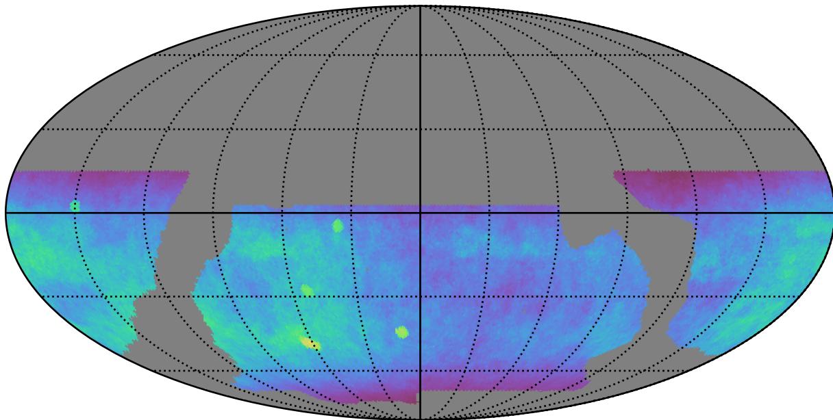
baseline_v2.0_10yrs WFD z band: Normalized Teff
