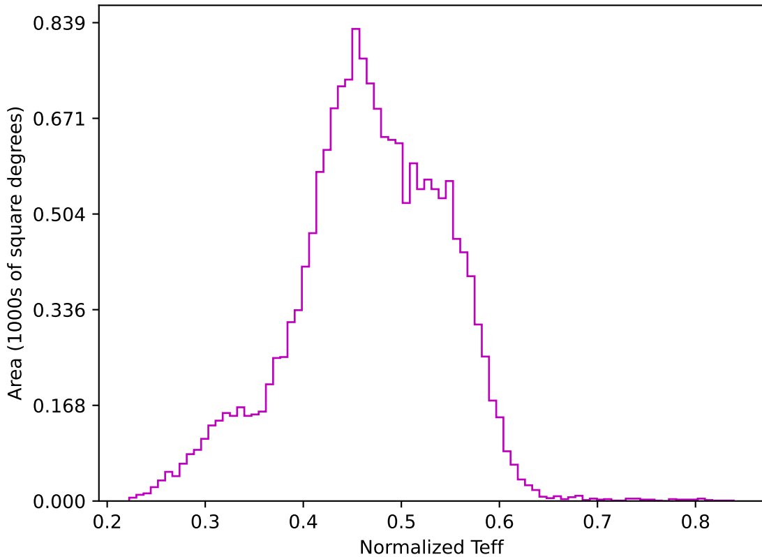
baseline_v2.0_10yrs WFD z band: Normalized Teff
