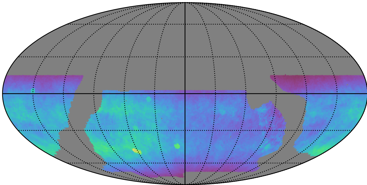
baseline_v2.0_10yrs WFD y band: Normalized Teff
