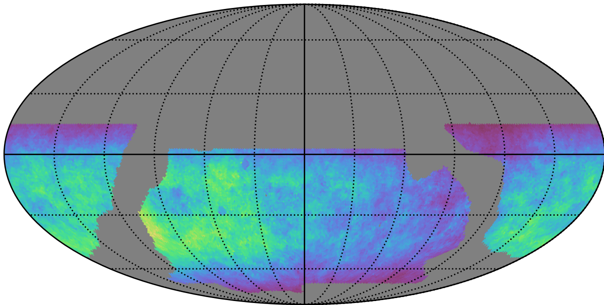
baseline_v2.0_10yrs WFD u band: Normalized Teff
