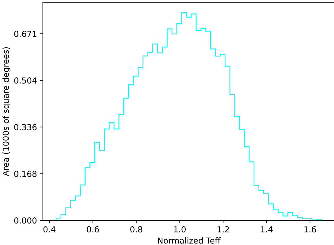
baseline_v2.0_10yrs WFD u band: Normalized Teff
