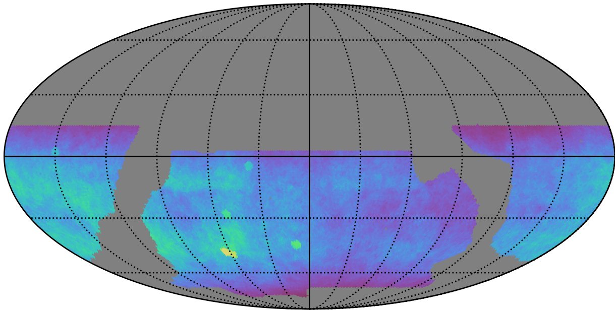
baseline_v2.0_10yrs WFD i band: Normalized Teff
