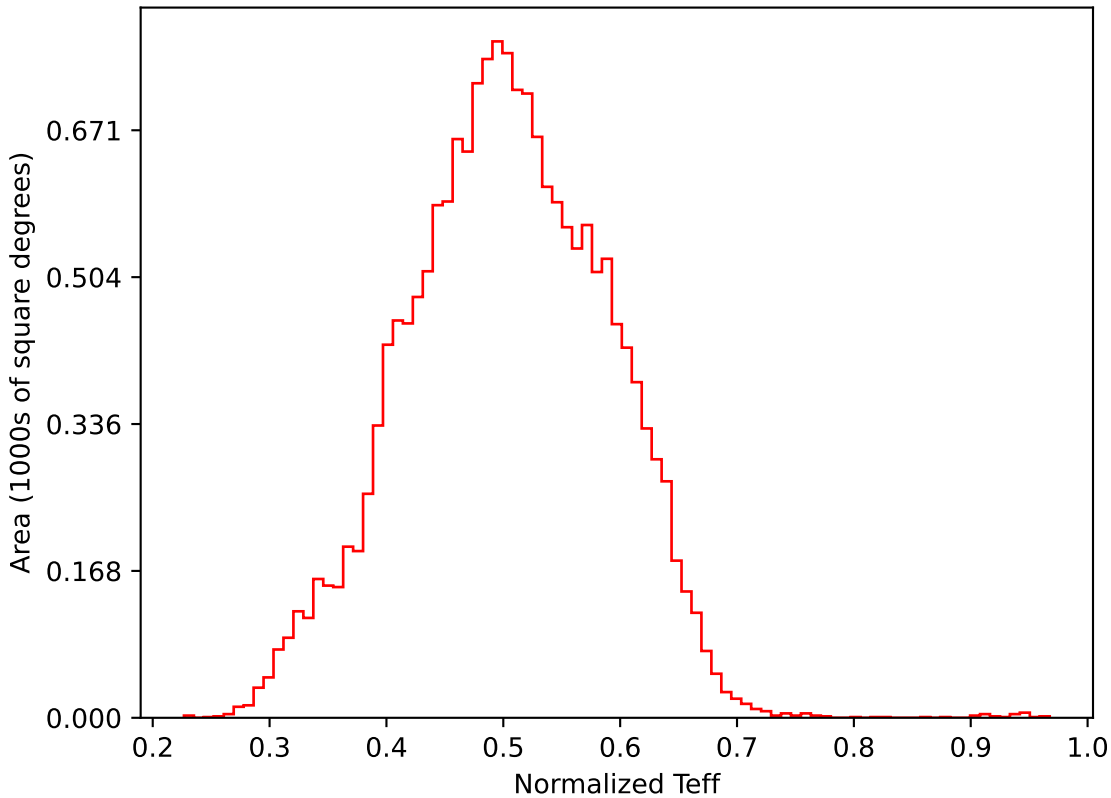
baseline_v2.0_10yrs WFD i band: Normalized Teff
