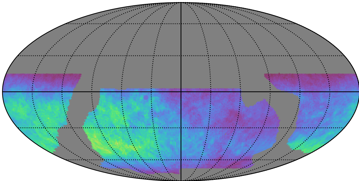
baseline_v2.0_10yrs WFD g band: Normalized Teff
