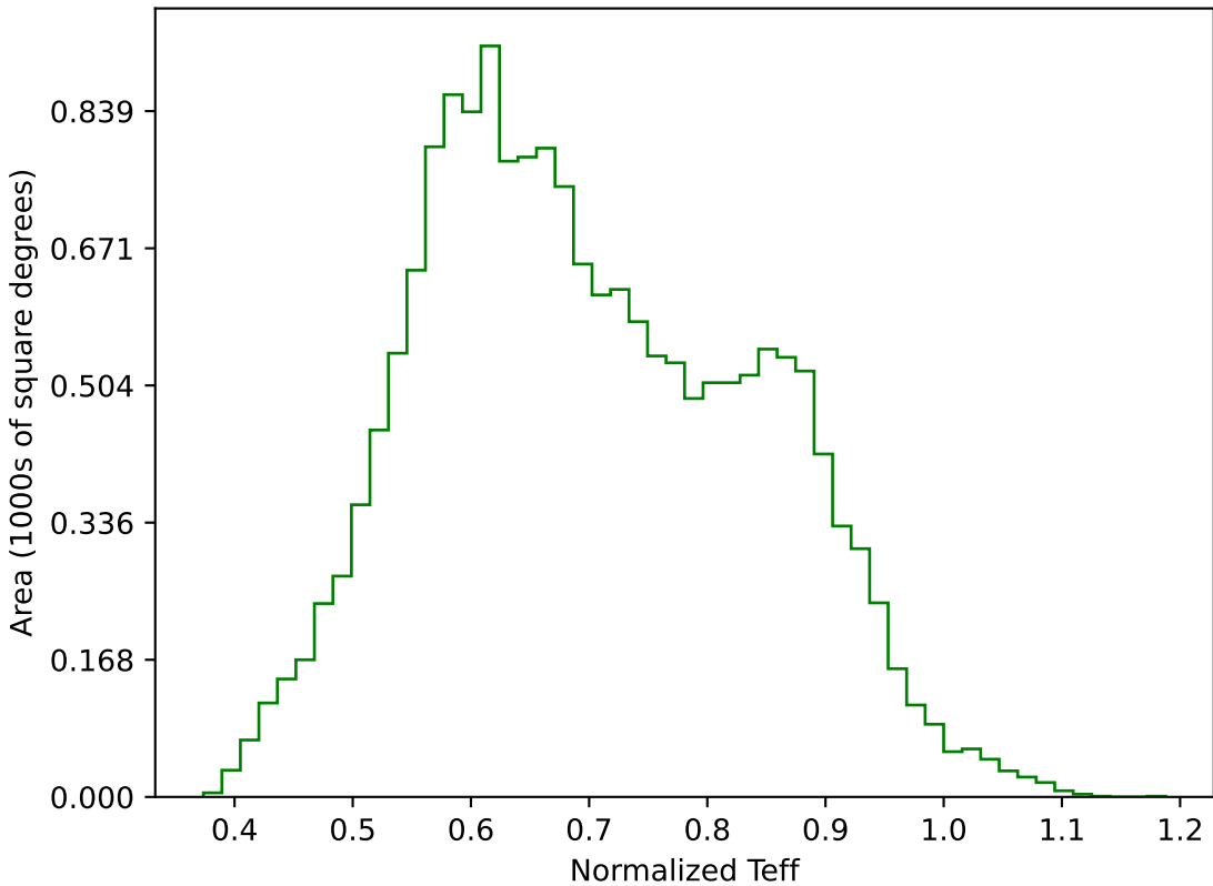
baseline_v2.0_10yrs WFD g band: Normalized Teff
