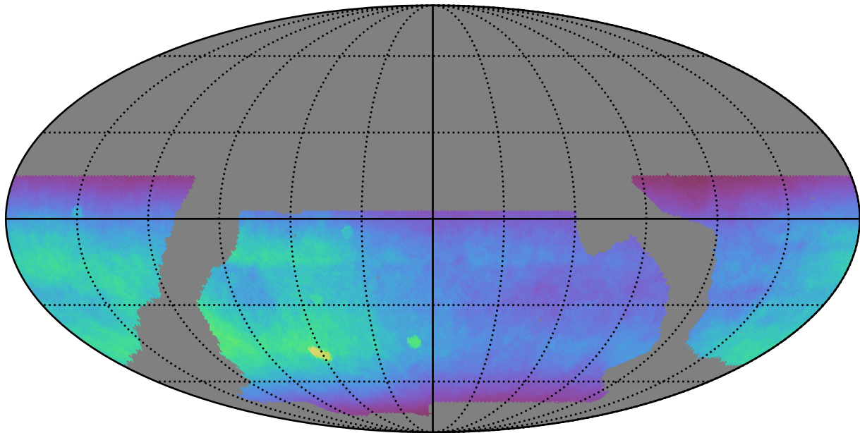
baseline_v2.0_10yrs WFD all bands: Normalized Teff
