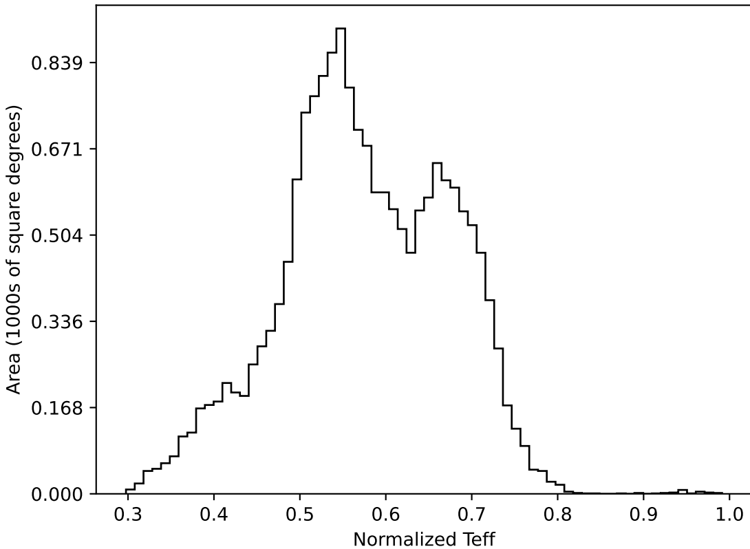
baseline_v2.0_10yrs WFD all bands: Normalized Teff
