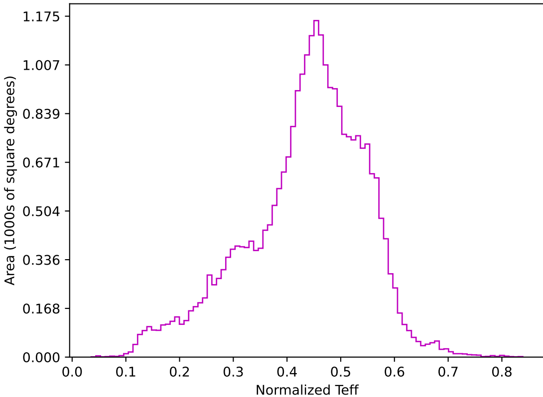
baseline_v2.0_10yrs All sky z band: Normalized Teff
