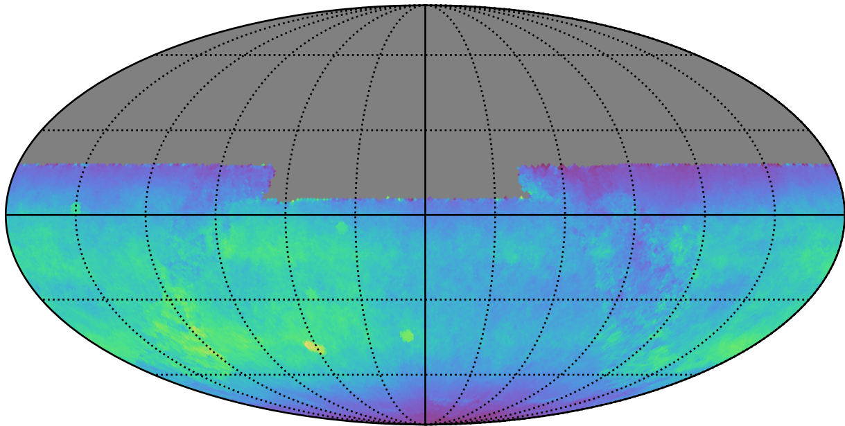
baseline_v2.0_10yrs All sky y band: Normalized Teff
