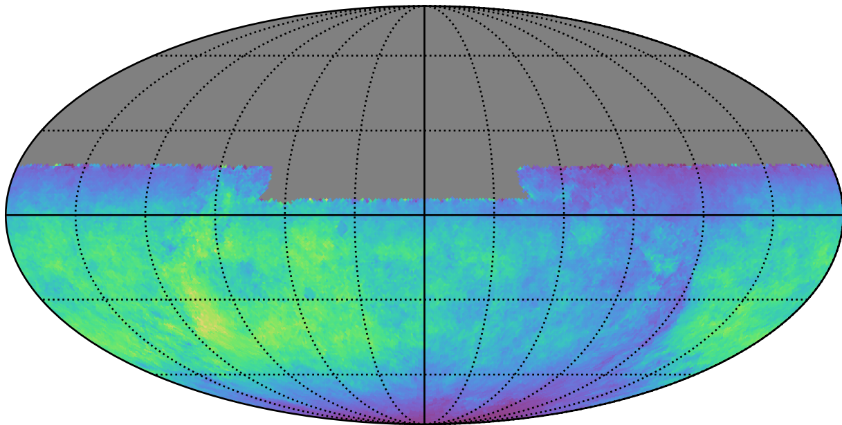
baseline_v2.0_10yrs All sky u band: Normalized Teff
