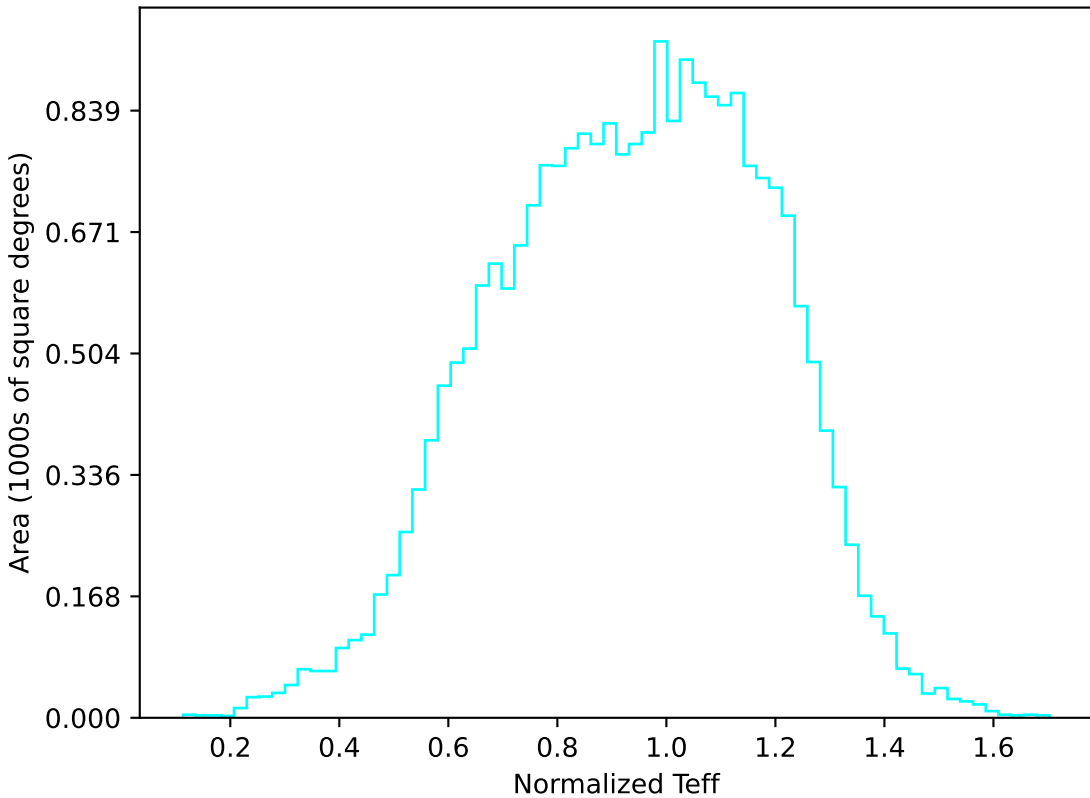
baseline_v2.0_10yrs All sky u band: Normalized Teff
