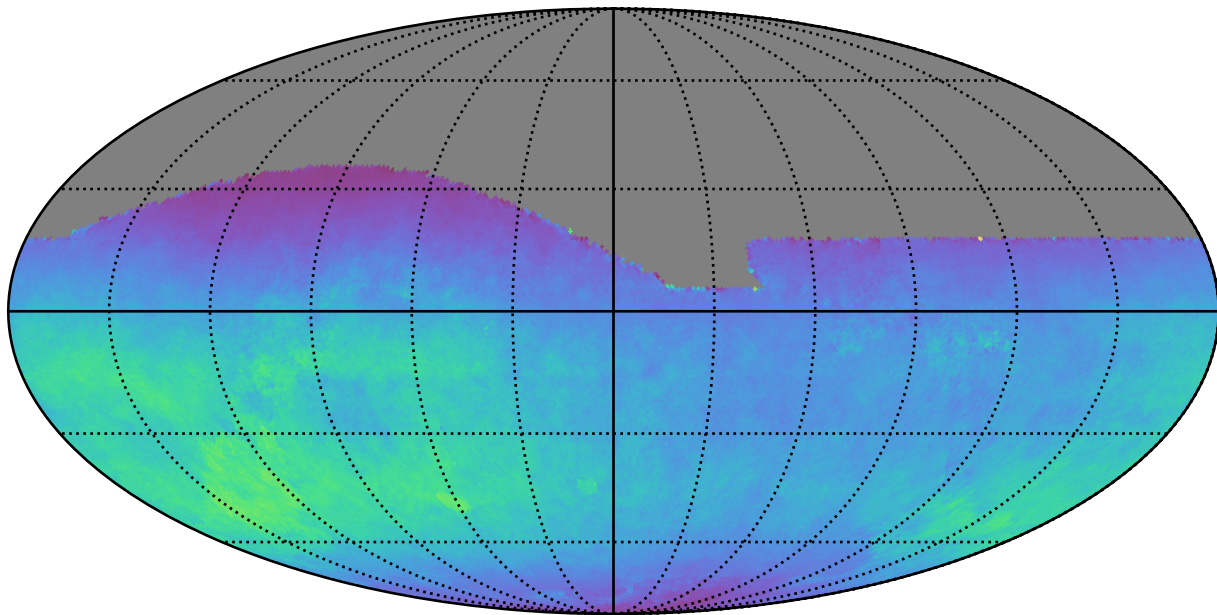
baseline_v2.0_10yrs All sky r band: Normalized Teff
