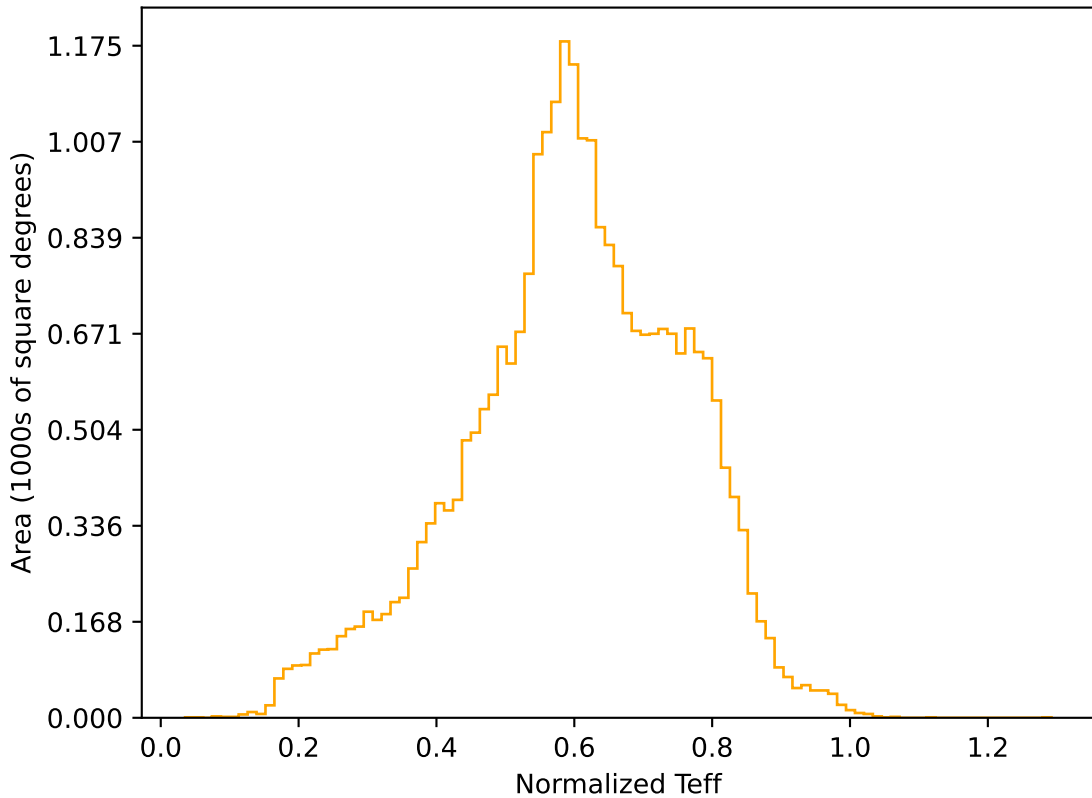
baseline_v2.0_10yrs All sky r band: Normalized Teff
