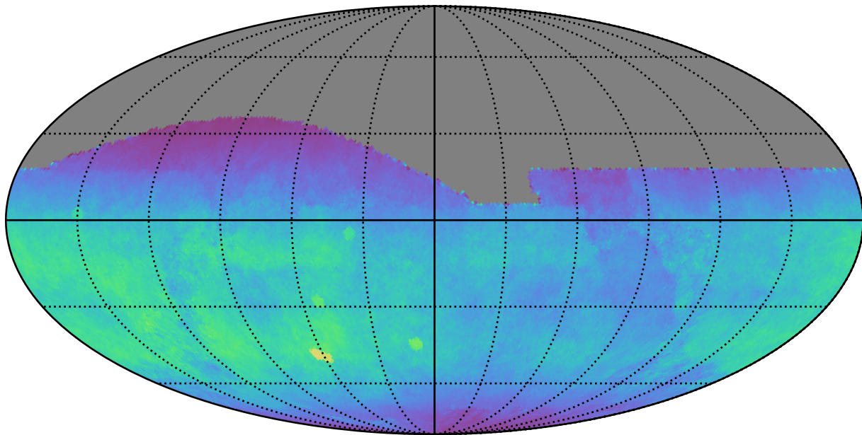
baseline_v2.0_10yrs All sky i band: Normalized Teff
