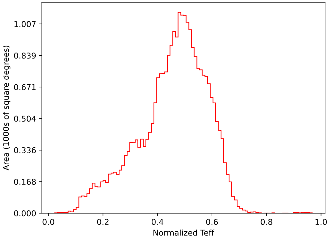
baseline_v2.0_10yrs All sky i band: Normalized Teff
