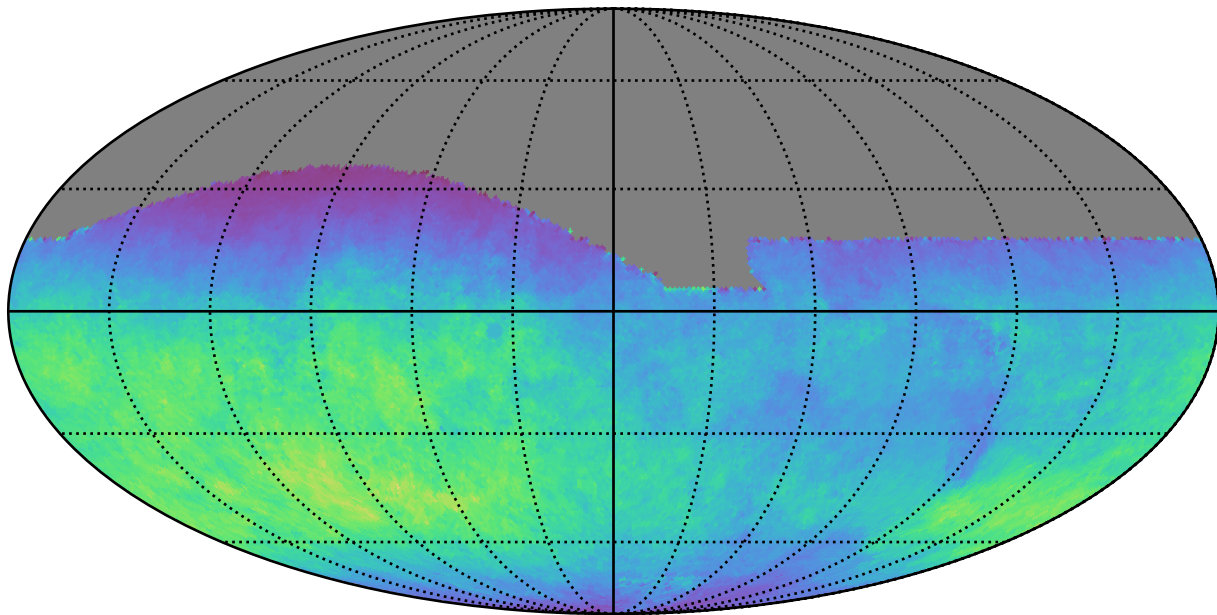
baseline_v2.0_10yrs All sky g band: Normalized Teff
