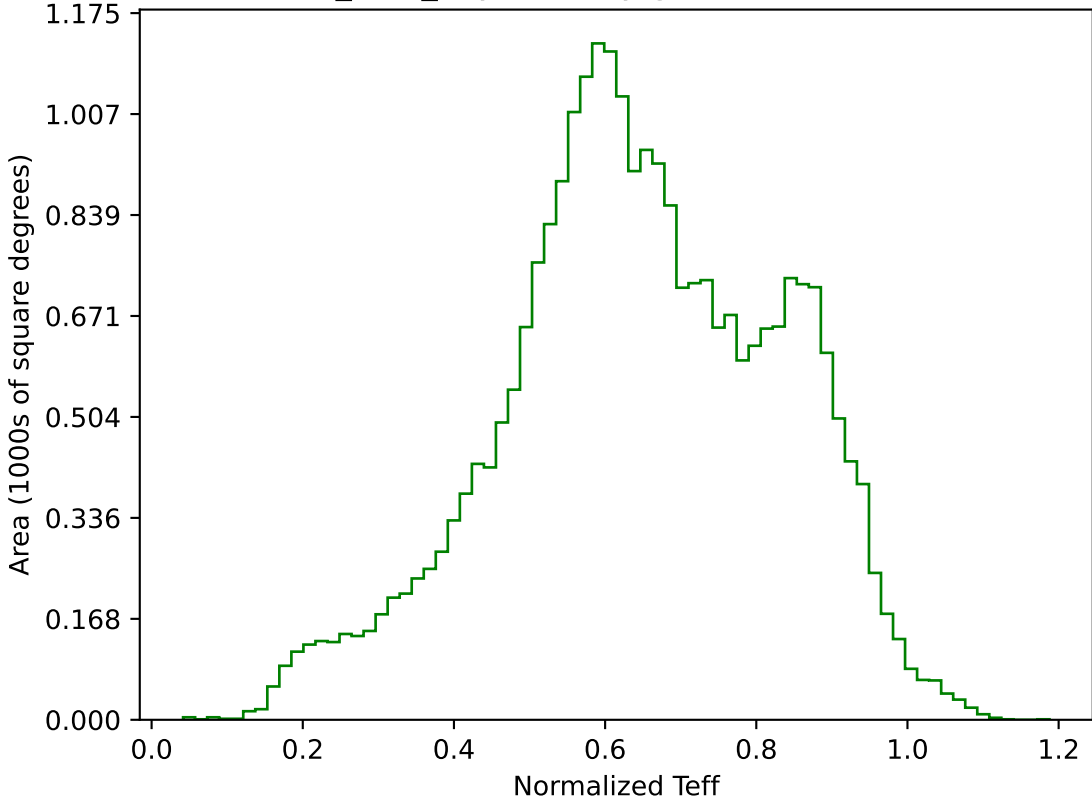
baseline_v2.0_10yrs All sky g band: Normalized Teff
