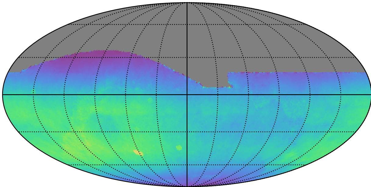
baseline_v2.0_10yrs All sky all bands: Normalized Teff
