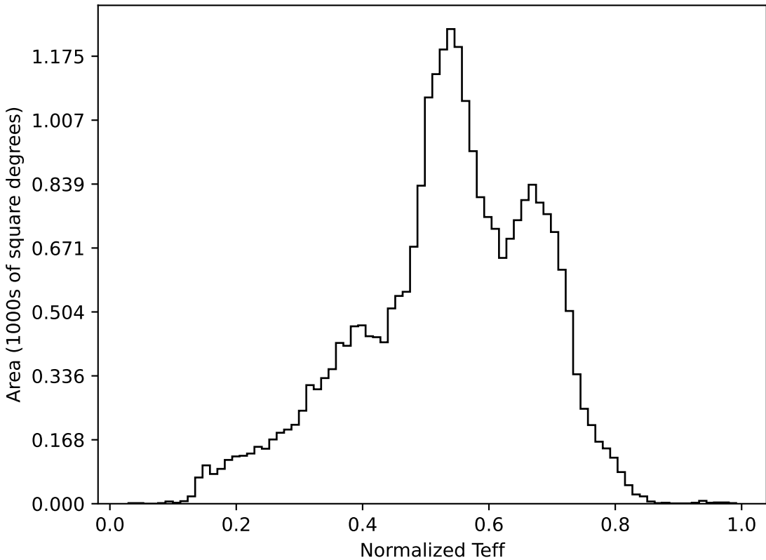
baseline_v2.0_10yrs All sky all bands: Normalized Teff
