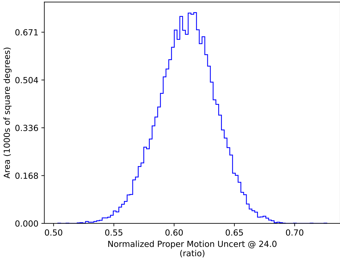
baseline_v2.0_10yrs WFD: Normalized Proper Motion Uncert @ 24.0
