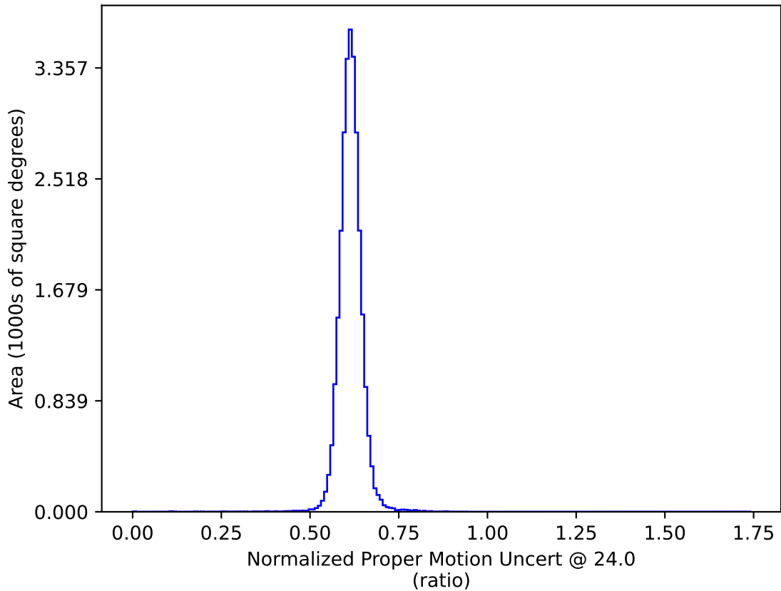
baseline_v2.0_10yrs All sky: Normalized Proper Motion Uncert @ 24.0
