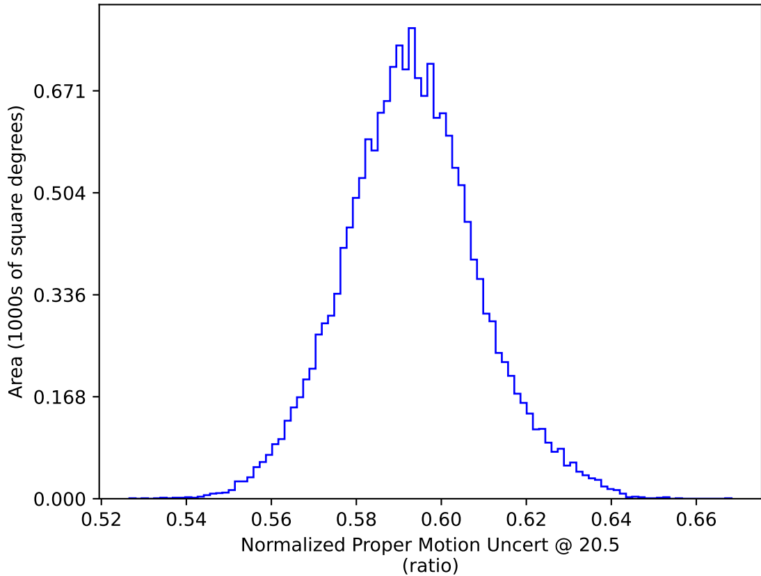
baseline_v2.0_10yrs WFD: Normalized Proper Motion Uncert @ 20.5
