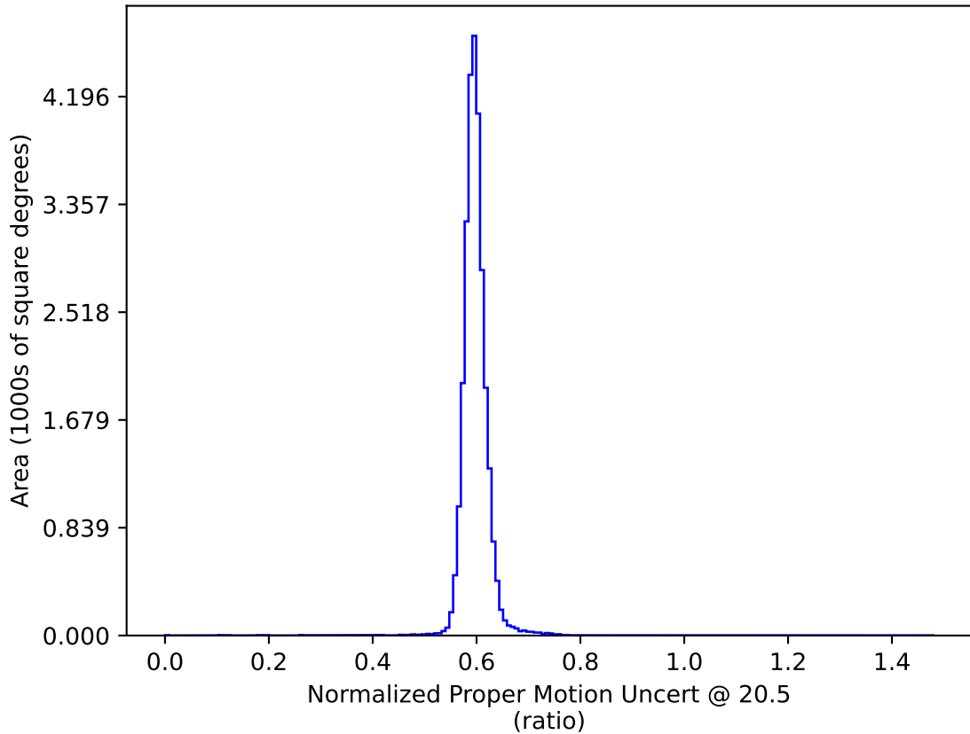
baseline_v2.0_10yrs All sky: Normalized Proper Motion Uncert @ 20.5
