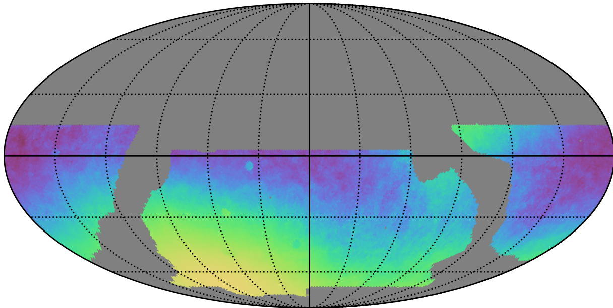
baseline_v2.0_10yrs WFD: Normalized Parallax Uncert @ 24.0
