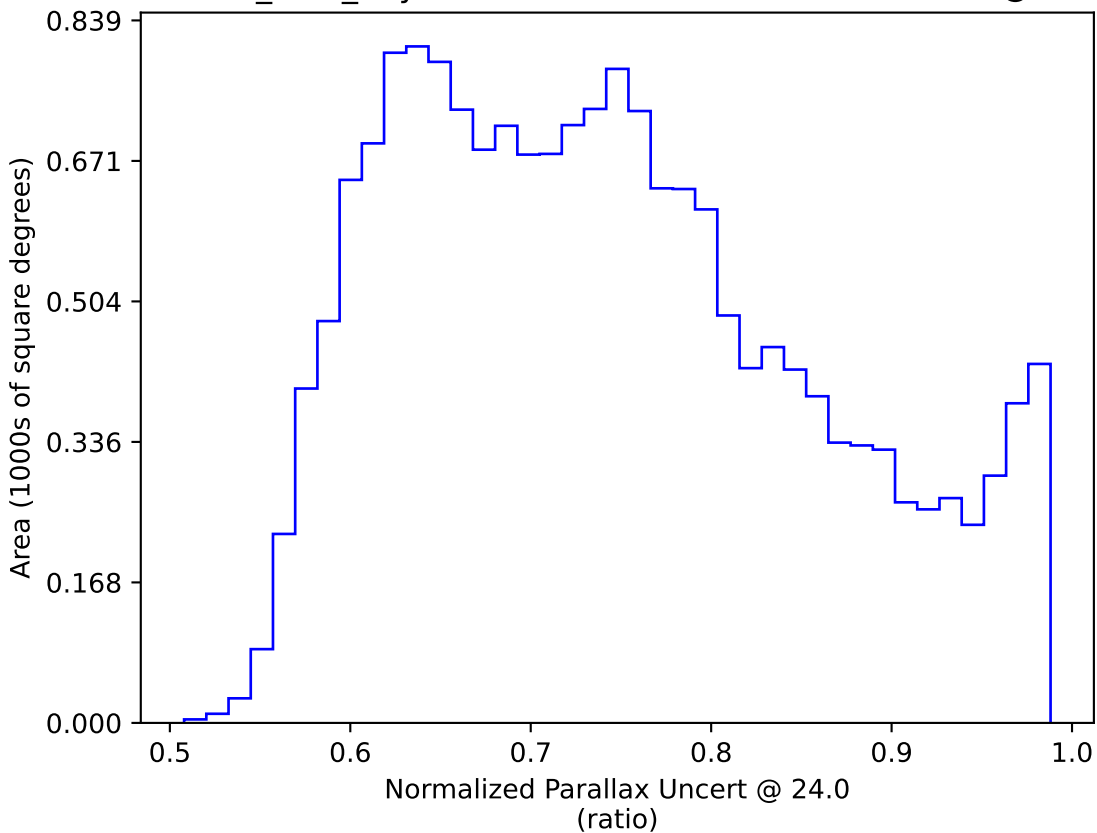
baseline_v2.0_10yrs WFD: Normalized Parallax Uncert @ 24.0
