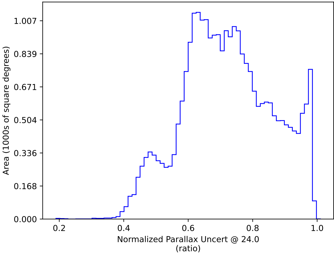
baseline_v2.0_10yrs All sky: Normalized Parallax Uncert @ 24.0
