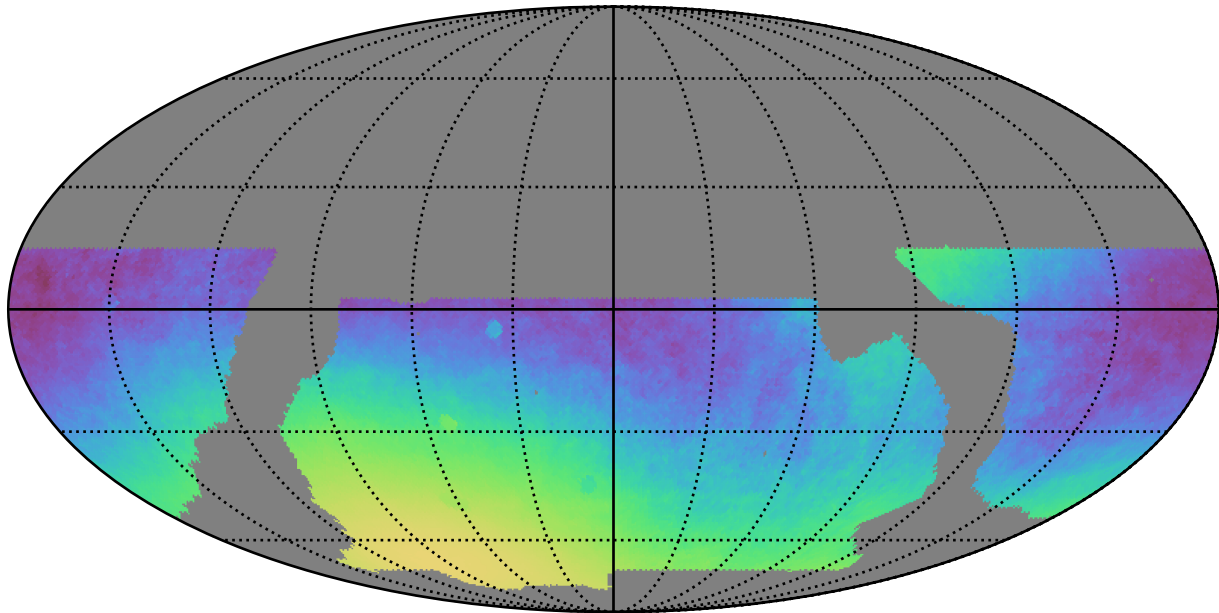
baseline_v2.0_10yrs WFD: Normalized Parallax Uncert @ 22.4
