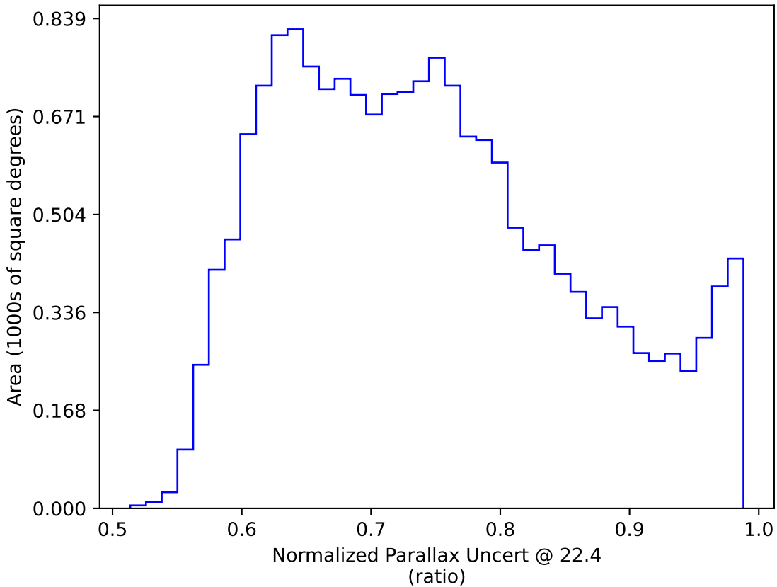
baseline_v2.0_10yrs WFD: Normalized Parallax Uncert @ 22.4
